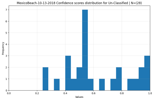
Figure: Confidence distribution for buildings labeled 'un-classified'.
