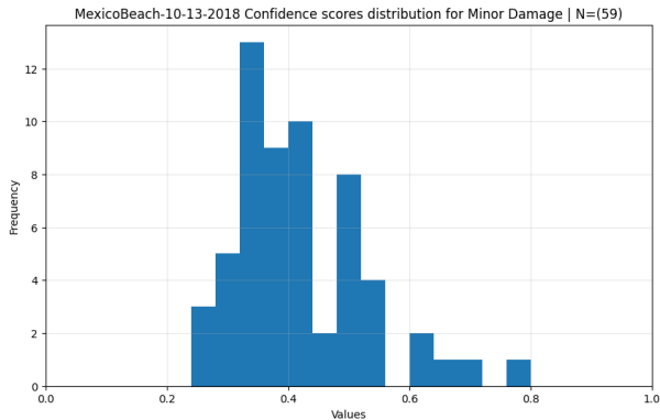
Figure: Confidence distribution for buildings labeled 'minor damage'.
